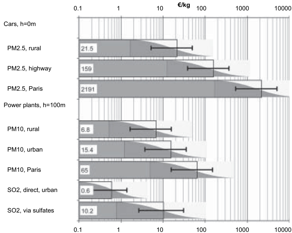
FIG. 2. Typical damage costs for PM and SO 2 (values of ExternE 1998 for France), together with the uncertainty range. The gray curve indicates the probability that the true cost is above a specified value. The mean damage costs are shown in the labels. On a log plot the distribution is symmetric about the median which is lower than the mean. The error bars indicate 1 geometric standard deviation (68% confidence interval).
