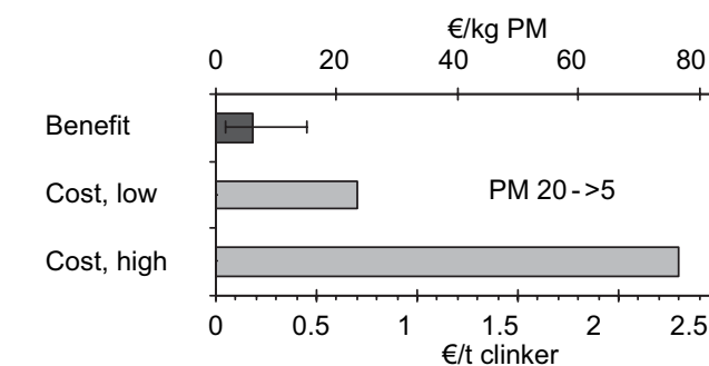
FIG. 3. Comparison benefits for a reduction of average emission from 20 to 5 \text{ mg}/\text{m}^3 (of emission limit from 50 to 15 \text{ mg}/\text{m}^3 ). Costs and benefits are shown on two scales: per \text{ton}_{\text{clinker}} (bottom) and per \text{kg}_{\text{PM}} (top). Error bar indicates uncertainty of benefit.
