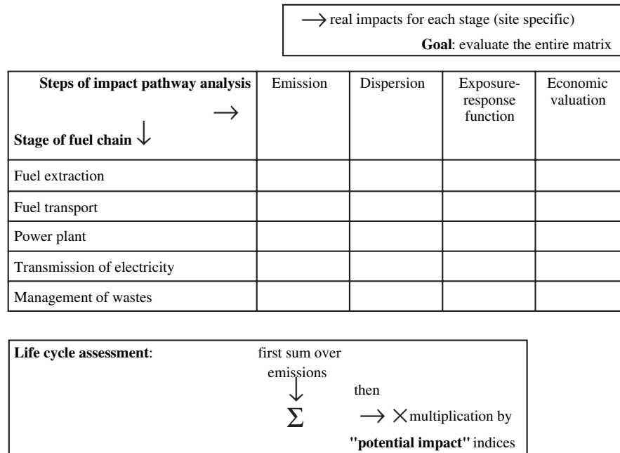
FIG. A1. Relation between impact pathway analysis and current practice of most LCA, illustrated for the example of electricity production From Spadaro and Rabl (1999).
