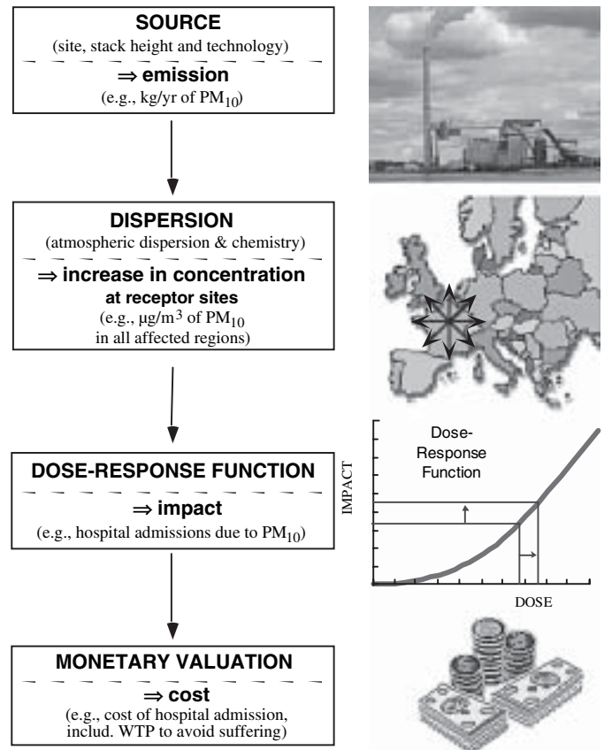
FIG. 1. Impact pathway analysis for the example of an air pollutant.
